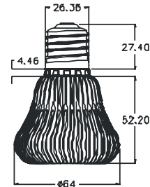
RTP-FPAR20-5X1.2W-002
