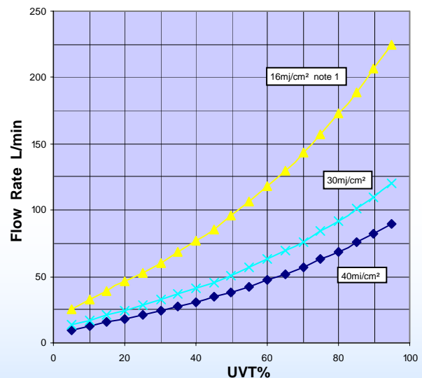
UVD1000 Performance Curves note 2
